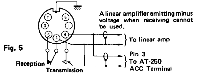
Rear view of the connector
